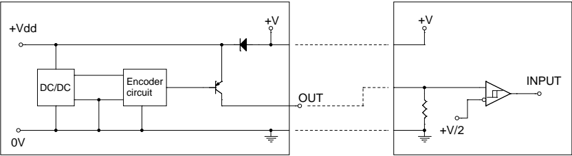
Recommended input circuit
