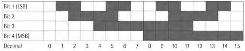
Gray code 4-bit representation (high logic level is represented in black)
