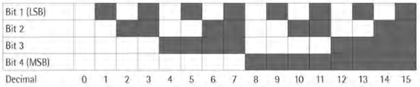
Binary code 4-bit representation (high logic level is represented in black)
